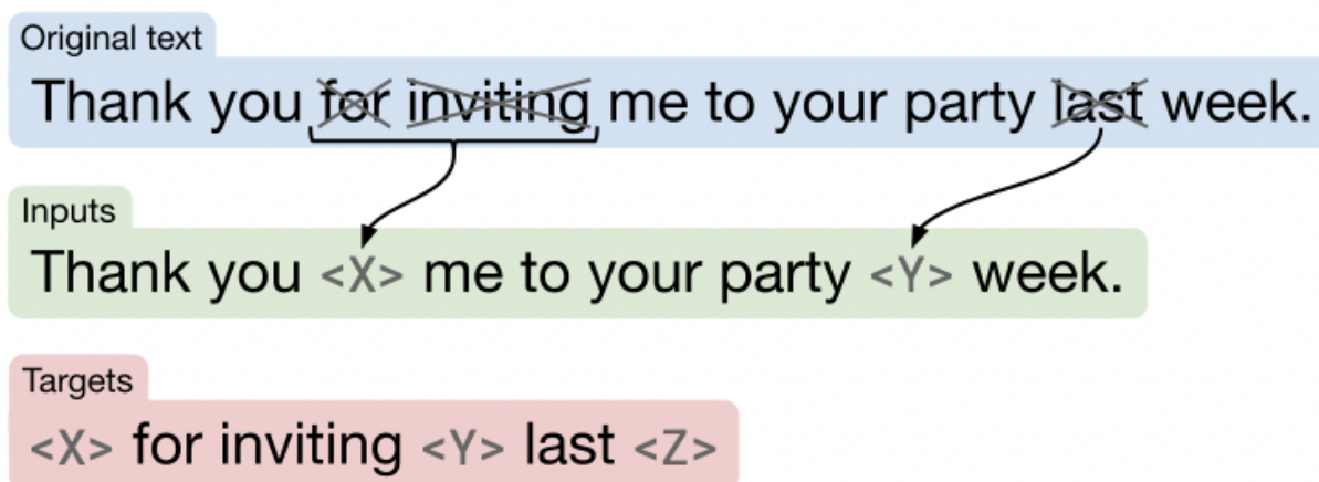
Figure 3: Example of how the BERT-style masked language modeling pretraining task is adapted to T5.
